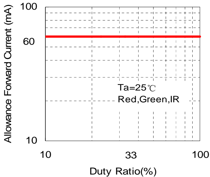
Figure 3. Duty Ratio vs Allowable Forward Current
