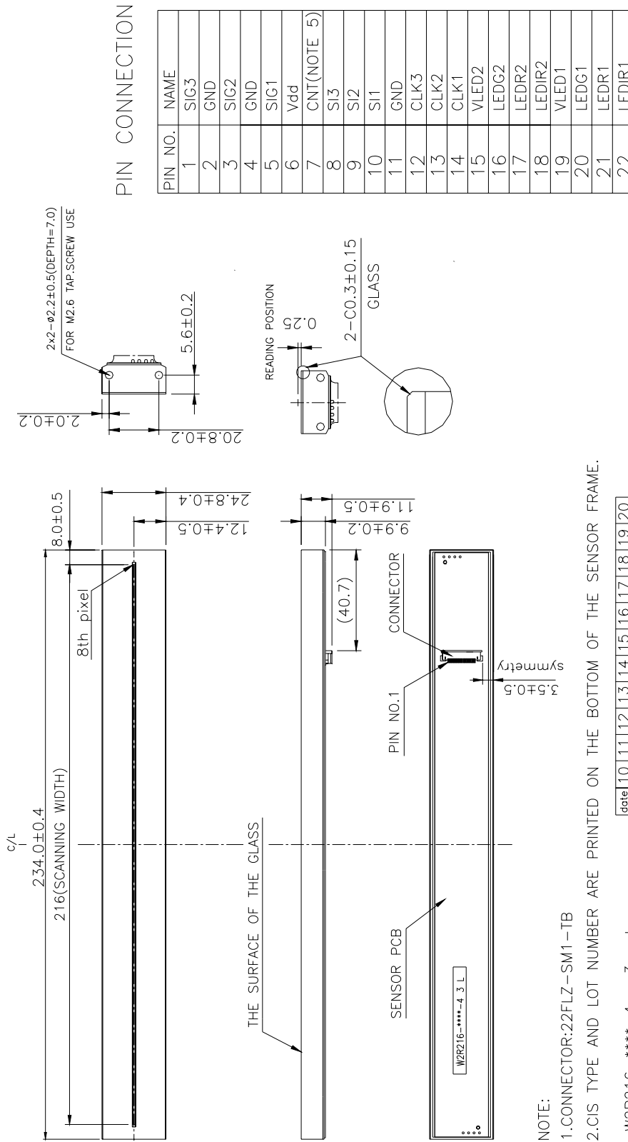
Figure 1 Dimensions
