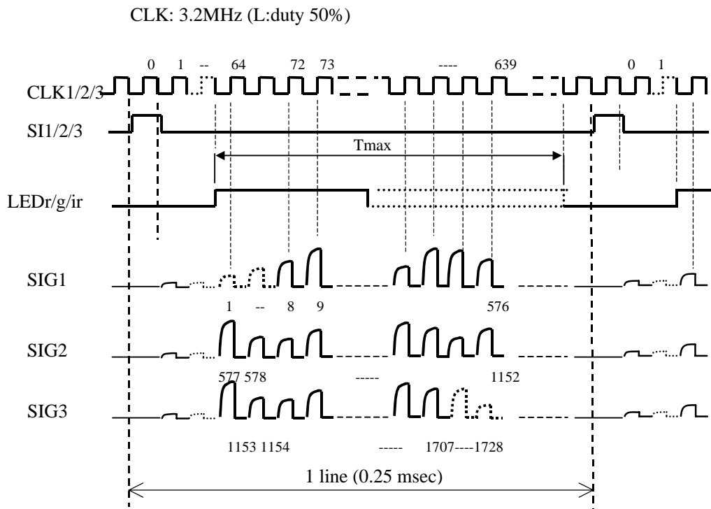
Figure 6. Timing Diagram
