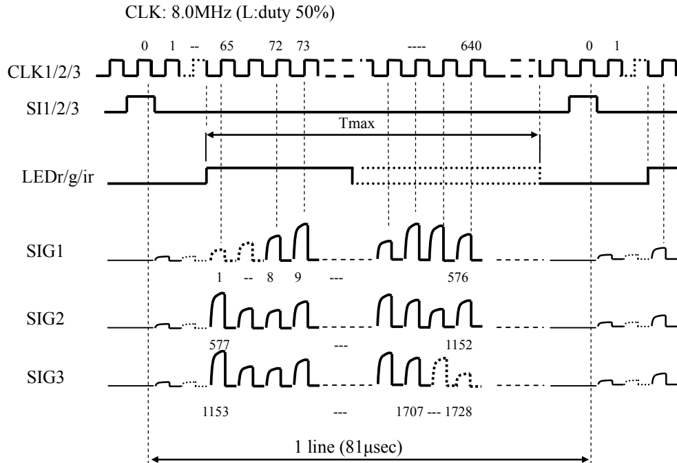
Figure 6. Timing Diagram (This is the SHEC shipping test condition.)
