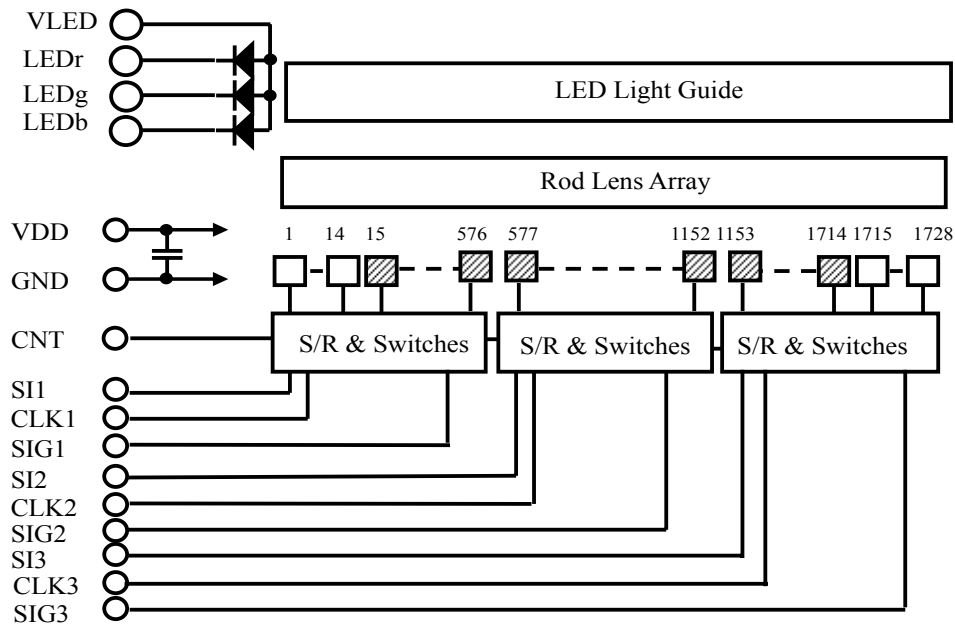
Figure 5. Block Diagram
