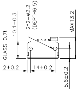
Figure 1 Dimensions
