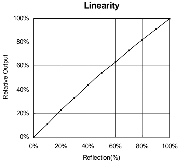
Figure 13. Typical Performance Curve Unless otherwise specified, Ta=25°
