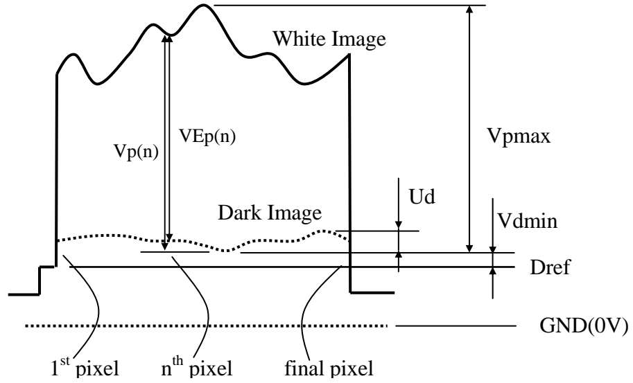
Figure 2. Output Signals Waveform
