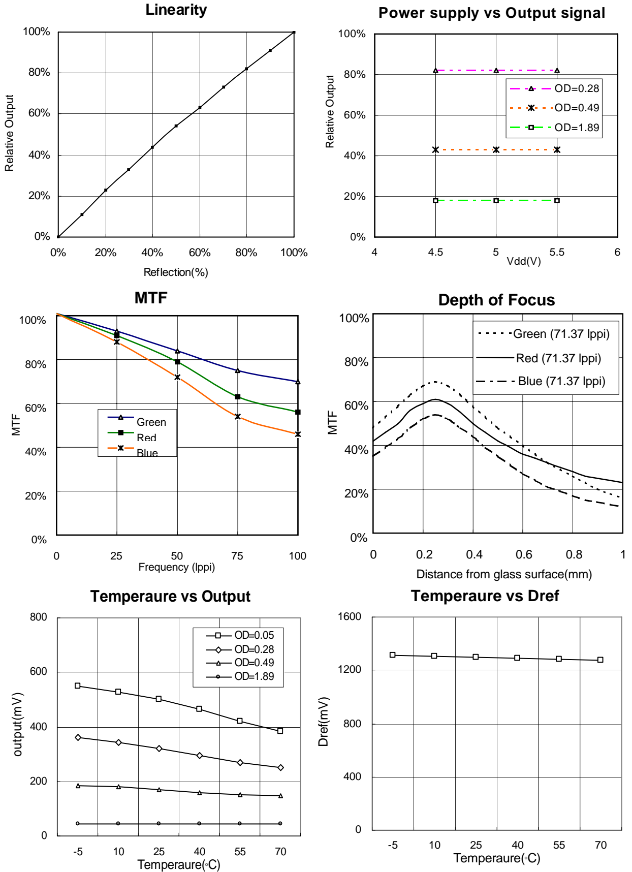
Figure 13. Typical Performance Curve Unless otherwise specified, Ta=25°
