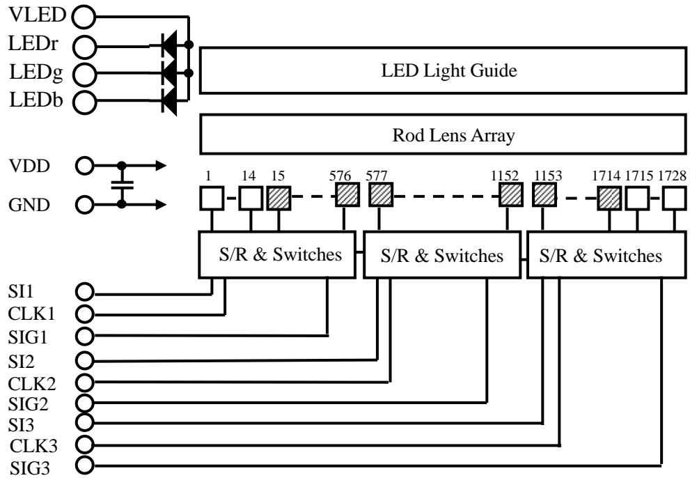
Figure 5. Block Diagram
