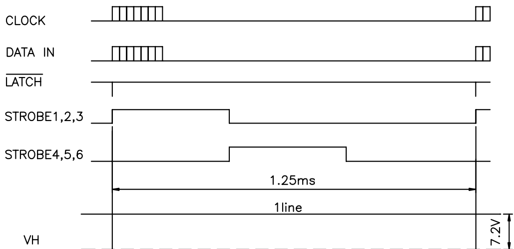
Fig. 2 Thermal Print Head (EN48N) Timing Chart
