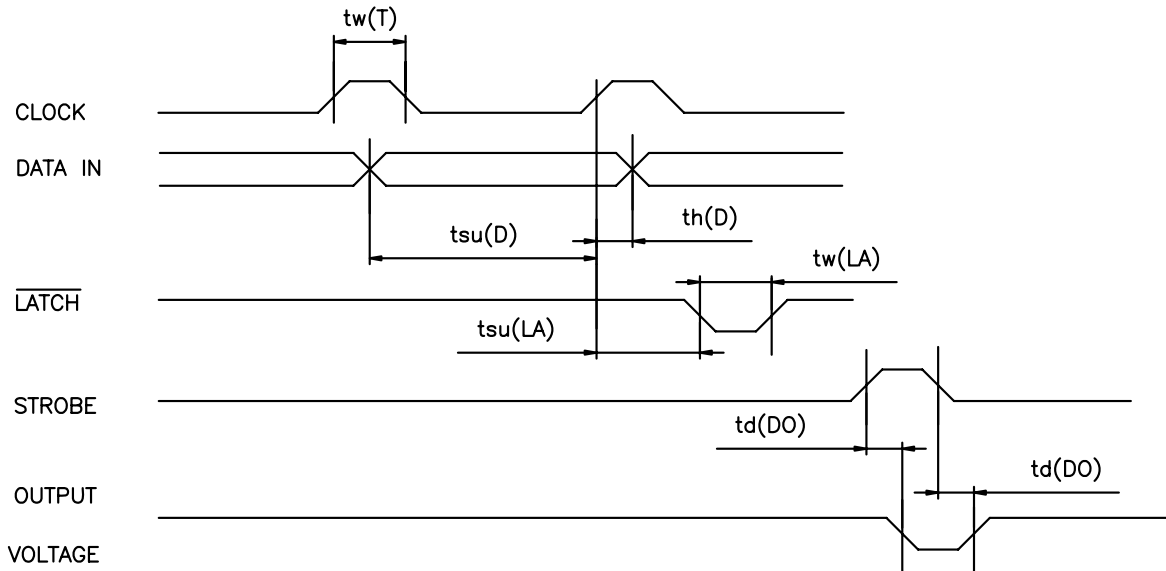
Fig. 2 Thermal Print Head (EN48N) Timing Chart
