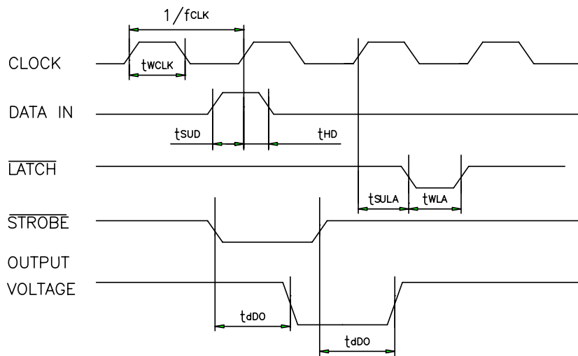
Fig. 2 Thermal Print Head (J8) Timing Chart
