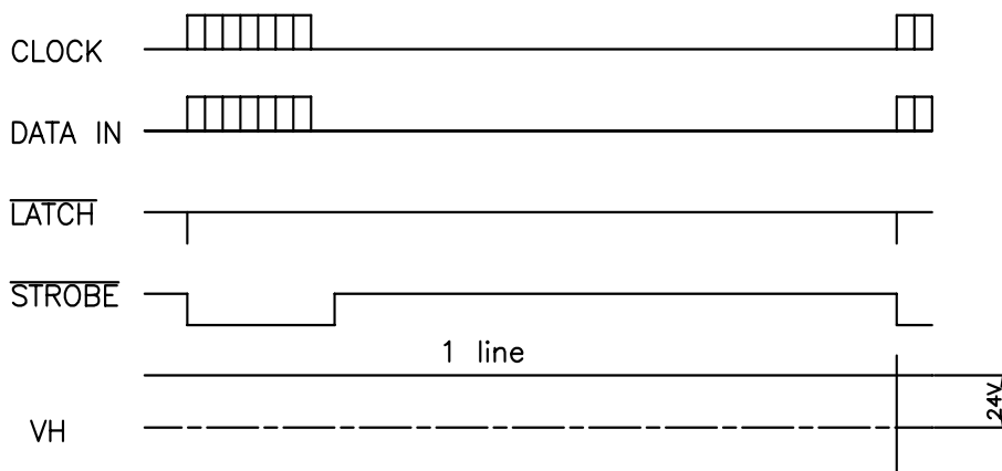
Fig. 2 Thermal Print Head (J8) Timing Chart
