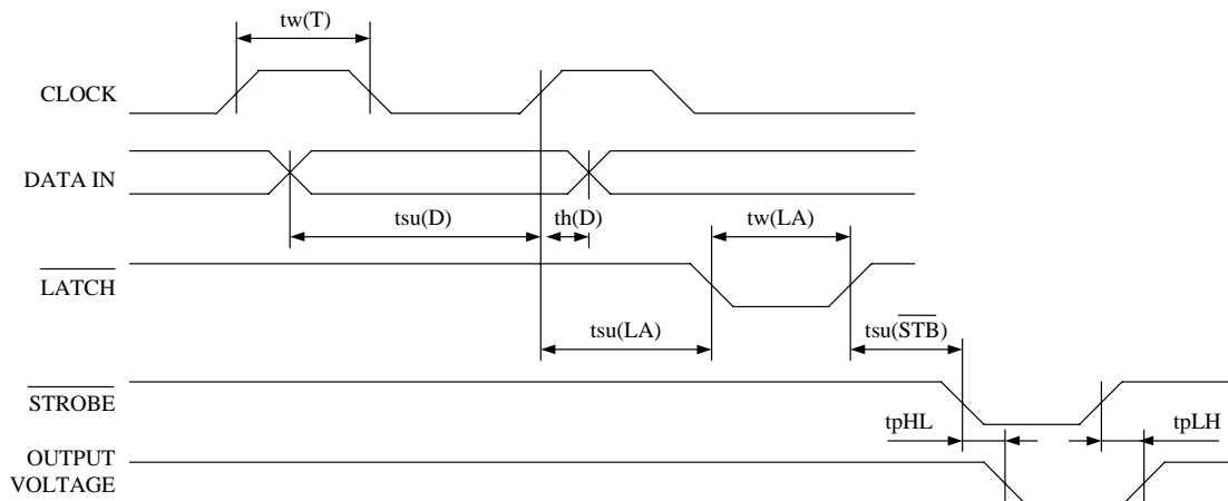
Fig. 2 Thermal Print Head (T80) Timing Chart
