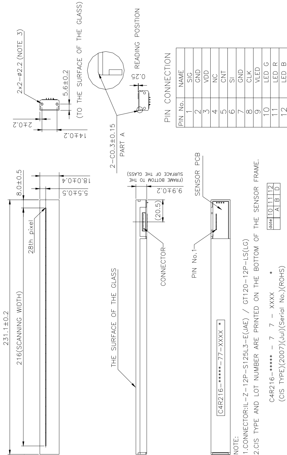
Figure 1 Dimensions
