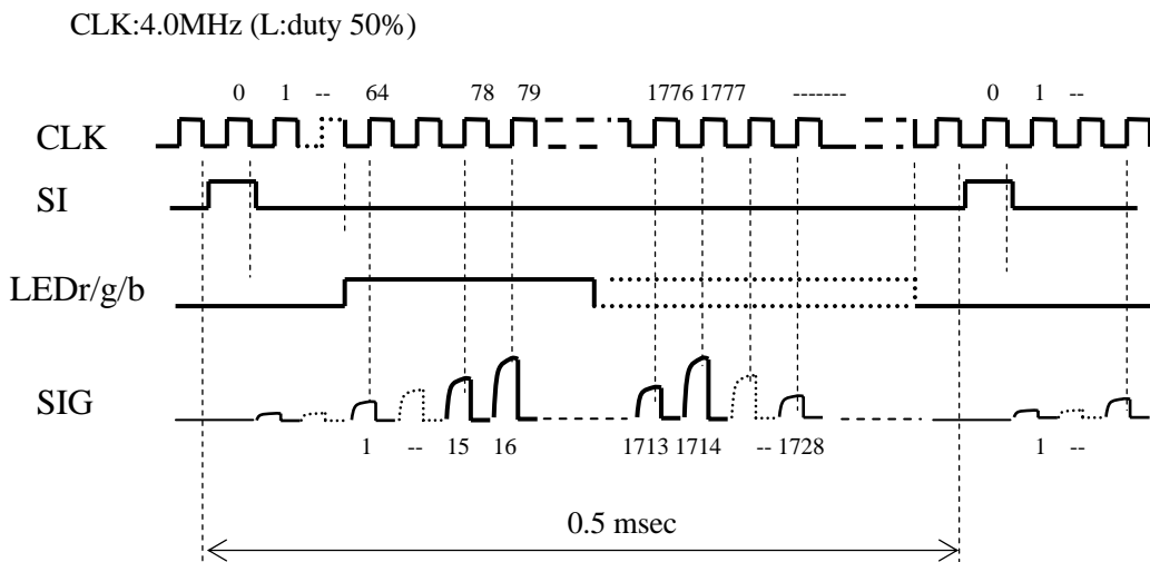
Figure 6. Timing Diagram
